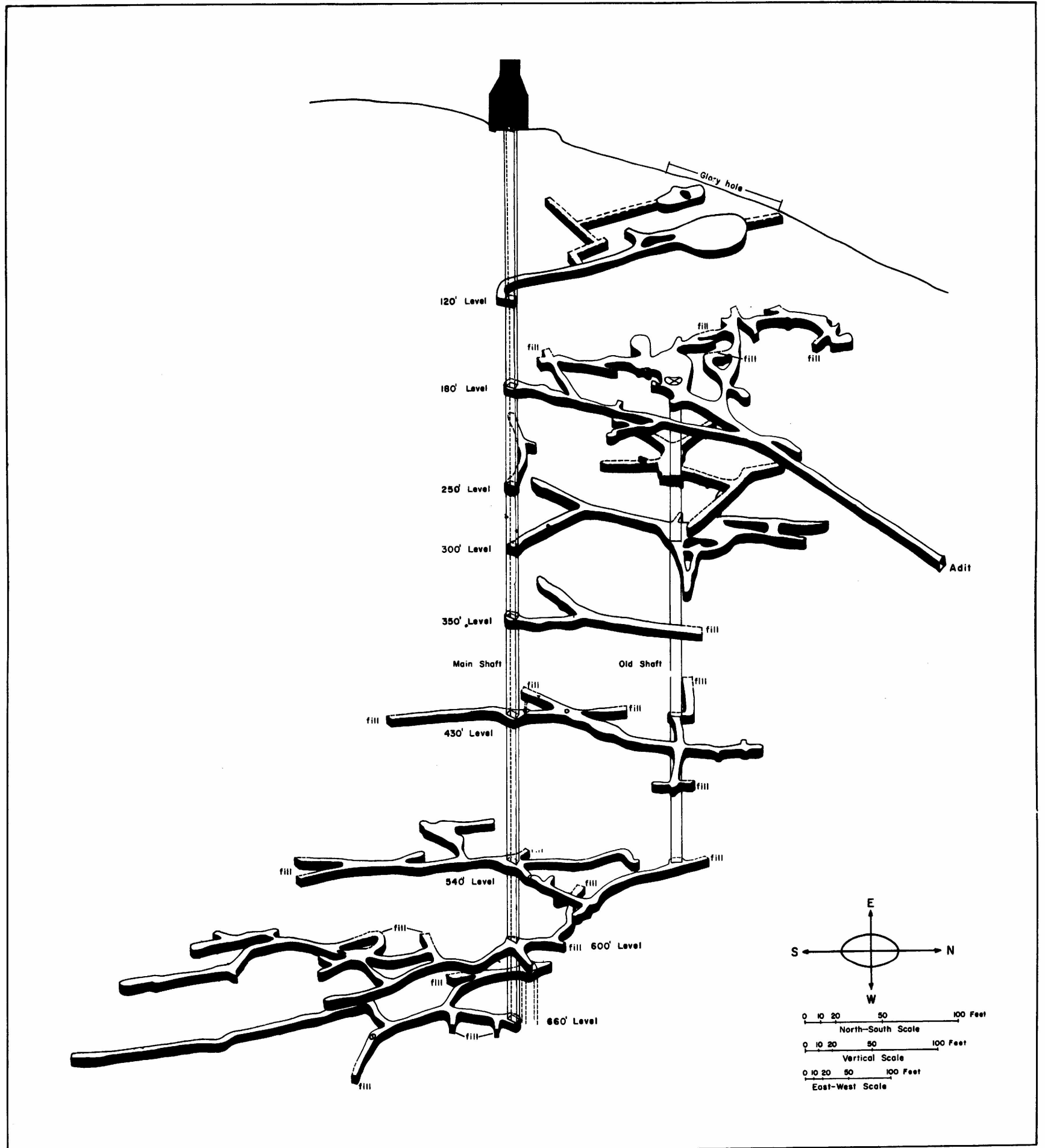
BLOCK DIAGRAM OF THE SOUTH HOMESTAKE MINE
